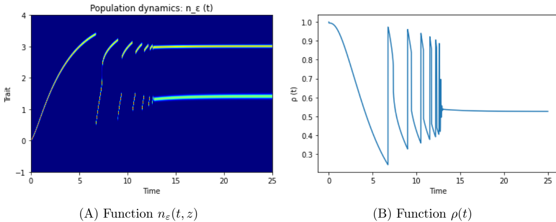
Figure 6: Solution u_\varepsilon of (42) in the dimorphic case \mu = 3.84 , with values \tau = 0.5 , g = 0.065 and \varepsilon = 5 \cdot 10^{-5} . The oscillations between maximum points stop in a finite time due to the small parameter \varepsilon > 0 .
