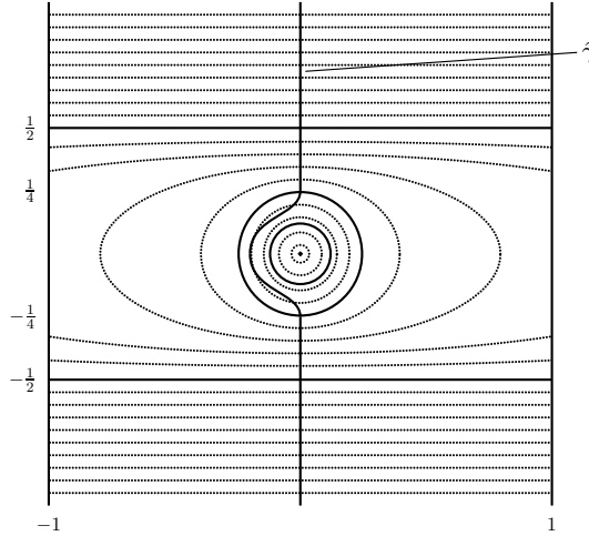
Figure 9: Sketch of vortex function s with ellipsoid level sets in the inner part.
