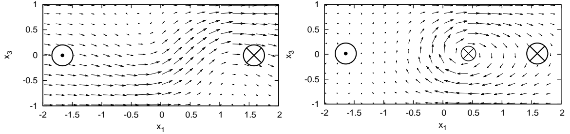
Figure 3: Asymmetric Néel wall (on the left) and asymmetric Bloch wall (on the right). Numerics. 7
