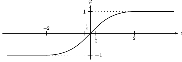
Figure 11: The non-linear change of variables \varphi .
