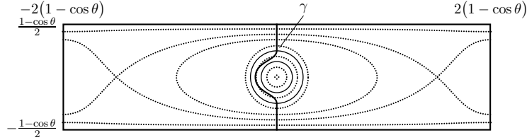
Figure 8: Enlargement of the area around the vortex, cf. Figure 7.
