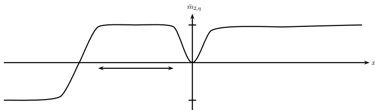
Figure 4: The x_3 -average \bar{m}_{2,\eta} of the m_2 -component. The arrow \longleftrightarrow denotes that the length of the corresponding interval grows to +\infty as \eta \downarrow 0 . Then the limit \bar{m}_2 (as \eta \downarrow 0 ) has the same sign at +\infty and -\infty .
