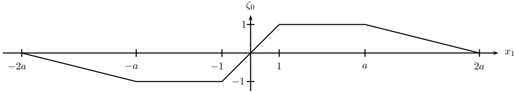
Figure 5: Test function \zeta_0
