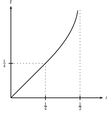
Figure 10: The semi-major axis t: (0, \frac{1}{2}) \rightarrow \mathbb{R} of the ellipses in Figure 9.
