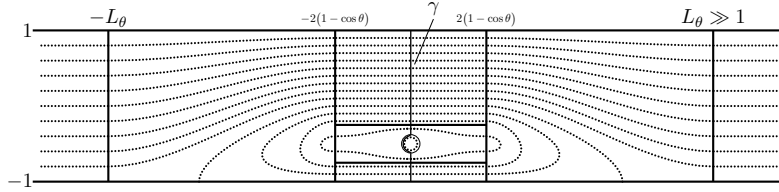
Figure 7: Sketch of the level lines of a stream function of an asymmetric domain wall of Bloch type.
