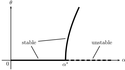
Figure 2: Bifurcation diagram for the angle \theta of the asymmetric core, depending on the global wall angle \alpha .
