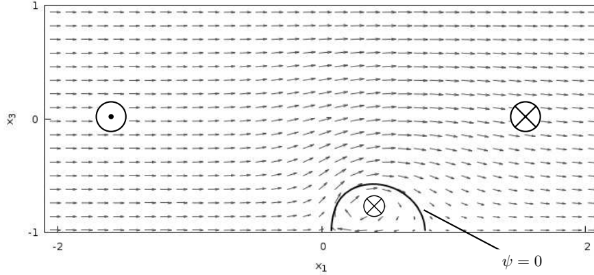
Figure 14: The zero level set of \psi for an asymmetric Bloch wall of angle \theta = 0.7 (cf. footnote in Fig. 3).
