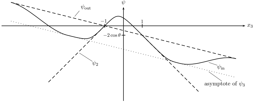
Figure 12: Sketch of the functions \psi_2(x_1, \cdot) (for |x_1| large, fixed) and \psi_{\text{out}} , as well as their interpolant \psi_{\text{in}} .
