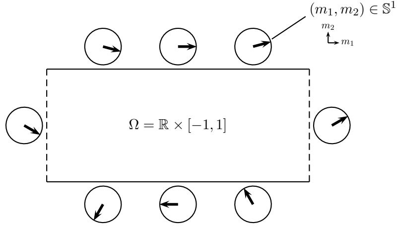
Figure 13: (m_1, m_2) on \partial\Omega .
