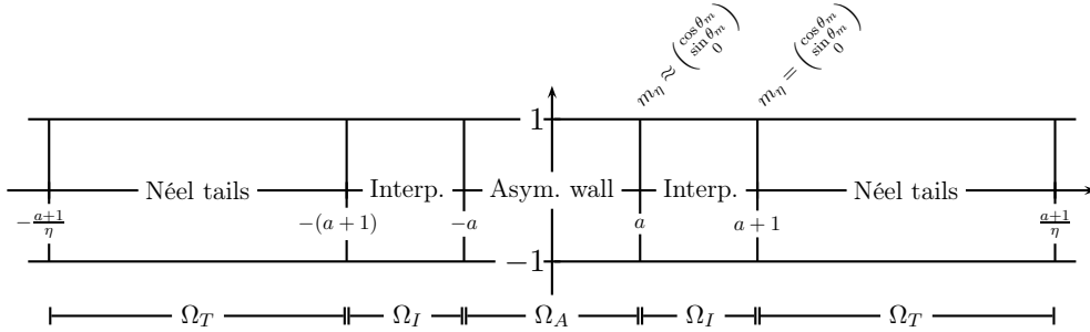
Figure 6: Construction of recovery sequence
