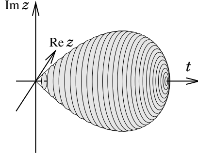
Figure 4: The surface of revolution over the nodal cubic
