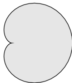
Figure 3: (1, 1)-hypercycle: an irrelevant solution to AlgDOP problem
