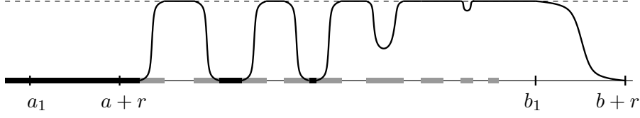
Figure 1: The graph of f_\varepsilon(t, 0) . Bold black: \Omega_{2\varepsilon} ; grey: \Omega \setminus \Omega_{2\varepsilon} .
