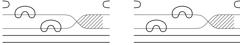
FIGURE 4. \mathcal{L}_p -schemes for Figure 2 (no. 44 in [4, Fig. 20]).
