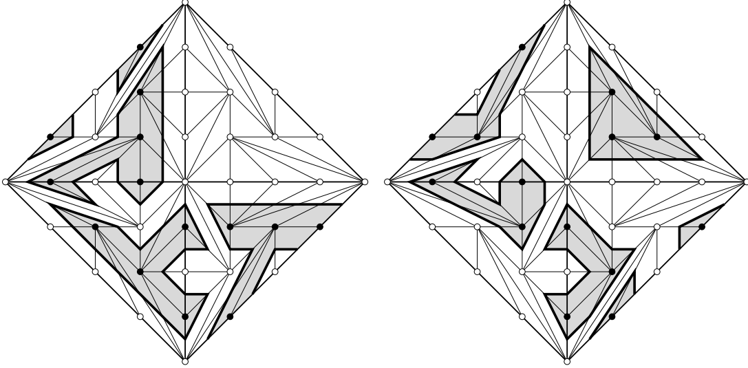
FIGURE 7. Patchworking of the arrangements in Figure 2.
