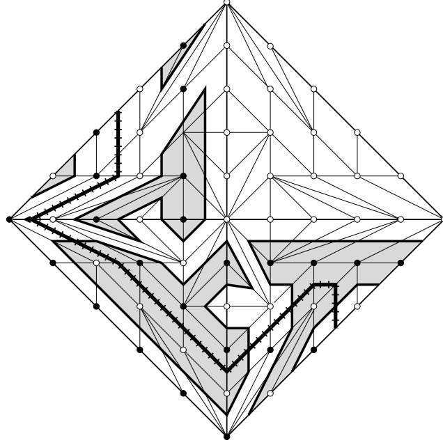
FIGURE 8. Patchworking with an additional line.
