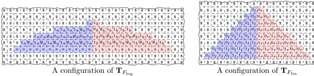
■ Figure 4 A configuration of \mathbf{T}_{F_{\log}} and \mathbf{T}_{F_{\text{lin}}} .
