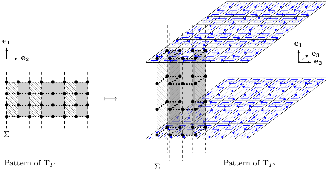
■ Figure 3 Pattern of \mathbf{T}_F wrapped following the tangled grid in a pattern of \mathbf{T}_{F'} .
