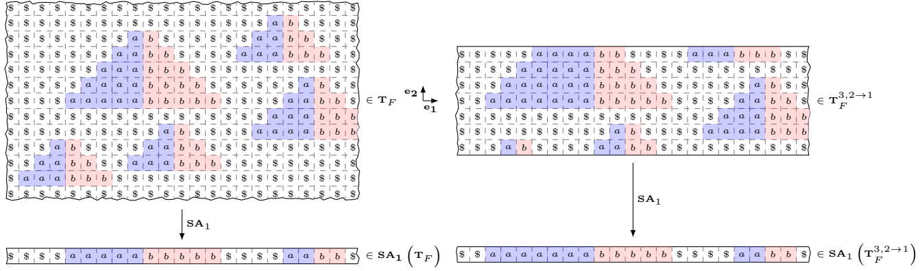
■ Figure 1 Application of \mathbf{SA}_1 under a configuration of \mathbf{T}_F and \mathbf{T}_F^{3,2 \rightarrow 1} .
