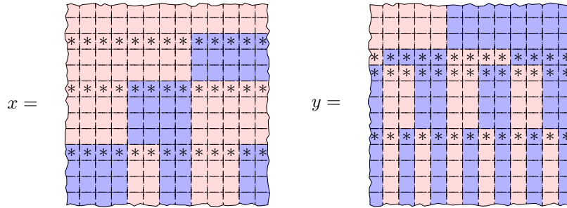
■ Figure 2 x and y are two examples of configurations of \mathbf{T}_{\text{Grid}} and y contains \infty (\square \blacksquare)^\infty .
