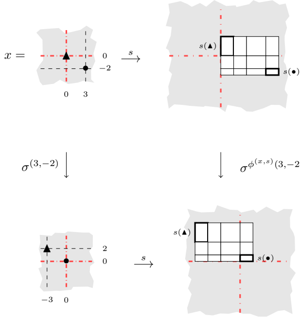
FIGURE 2. If the configuration x is compatible with the substitution s , then one can define the function \phi^{(x,s)} = \varphi^{(\mathbf{k}^{(s)}(x_{n,\dots,n}))}_{n \in \mathbb{Z}} which verifies s \circ \sigma^{\mathbf{i}}(x) = \sigma^{\phi^{(x,s)}(\mathbf{i})} \circ s(x) .
