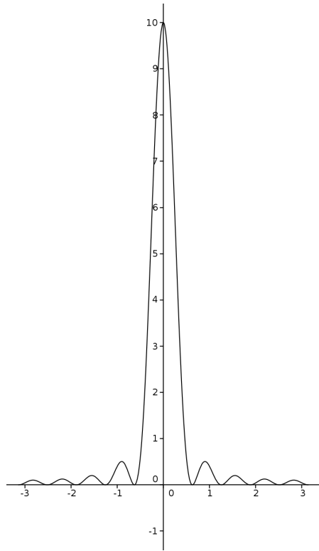
FIGURE 3.2 – K_{10}
