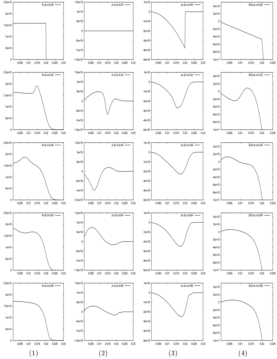
Fig. 1. Semi-Gaussian beam. Snapshots of slices of: (1) density N(t, r) , (2) first moment in v_r , (3) first moment in v_\theta , (4) total force field E_s(t, r) - \left(\frac{qB_z}{2m}\right)^2 r inside the beam at times z=0, 0.32, 0.48, 0.64, 0.96 m.
