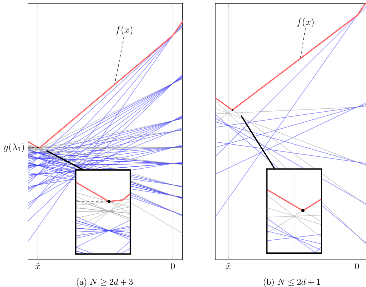
Figure 10 – The optimal value of the dual optimization problem lies at the intersection of the set of affine functions f_{\lambda,\mu}(x) . When N \geq 2d+3 (Figure 10a, with N = 9 and d = 3 ), then p^*(N, d) = g(\lambda_1) . When N \leq 2d + 1 (Figure 10b, with N = 5 and d = 3 ), then p^*(N, d) lies at the intersection of f_{\lambda_2, \mu_1} and f_{\lambda_1, \mu_2} . In ■ the max over all affine functions, in ■ the affine functions from the set \Gamma , and in ■ the affine functions from the set \Omega \setminus \Gamma .
