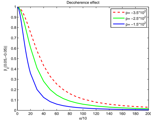
FIGURE 4. The quantity |I_\chi(0.05, -0.05)| as a function of \alpha for three different values of the momentum of the light particle.
