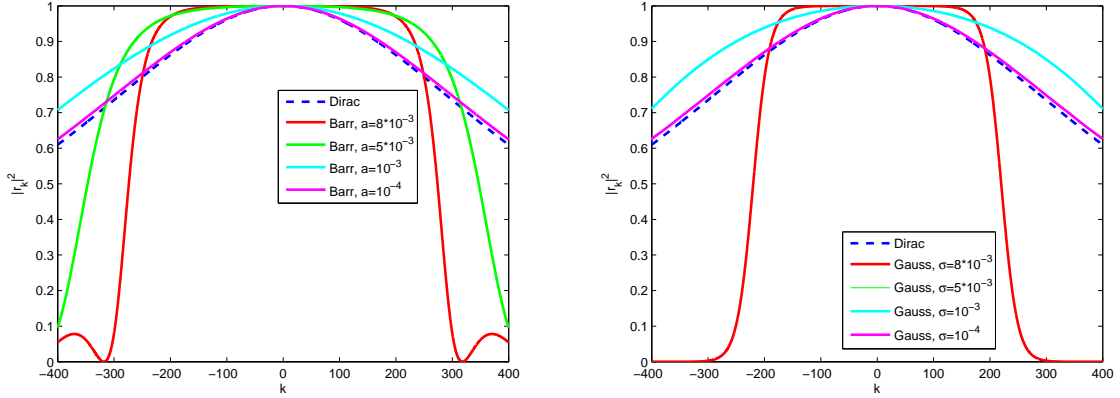
FIGURE 6. Comparison of the reflection amplitudes |r_k|^2 corresponding to three different interaction potentials, with fixed potential strength \alpha = 5 * 10^2 and various a and \sigma values. Left: Dirac's delta and potential barrier. Right: Dirac's delta and Gaussian potential.
