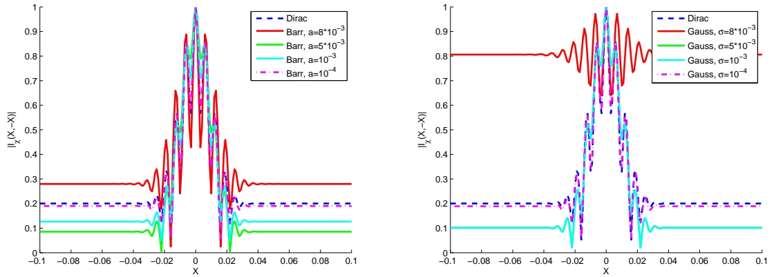
FIGURE 7. Comparison of the collision function I_\chi(X, -X) corresponding to three different interaction potentials, with fixed potential strength \alpha = 5 * 10^2 and various a and \sigma values. Left: Left: Dirac's delta and potential barrier. Right: Dirac's delta and Gaussian potential.
