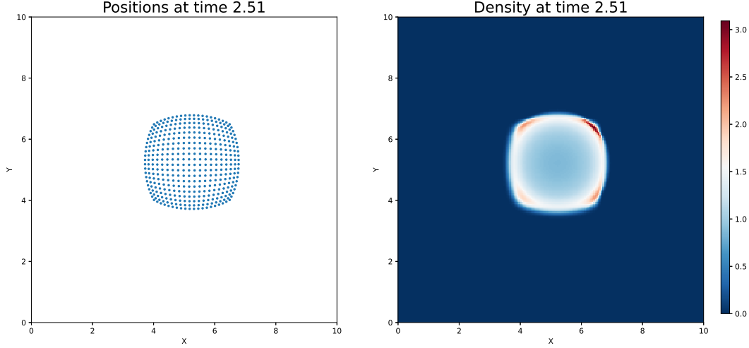
Figure 3.9: Drone swarm particle (left, N = 500 ) and fluid (right) simulations at t = 2.5s .
