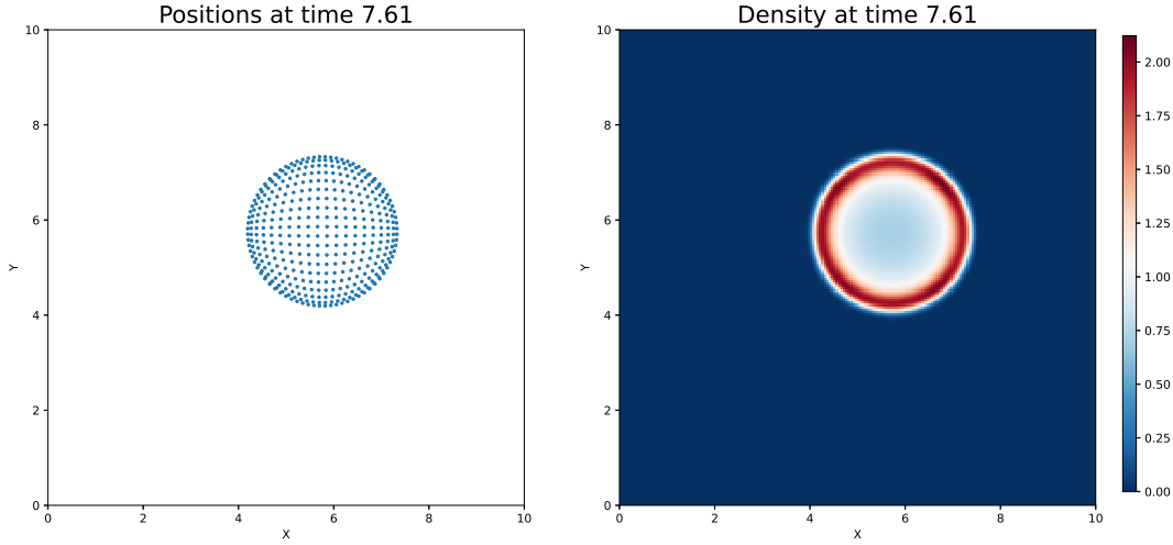
Figure 3.10: Drone swarm particle (left, N = 500 ) and fluid (right) simulations at t = 7.6s .
