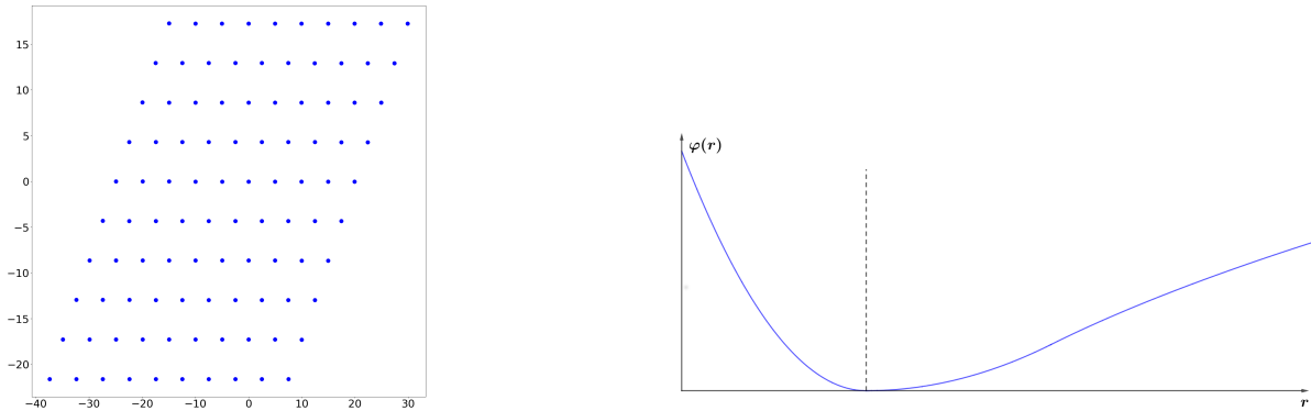
Figure 3.3: Uniform disc formation for the potential \varphi_{cris}(r) .
