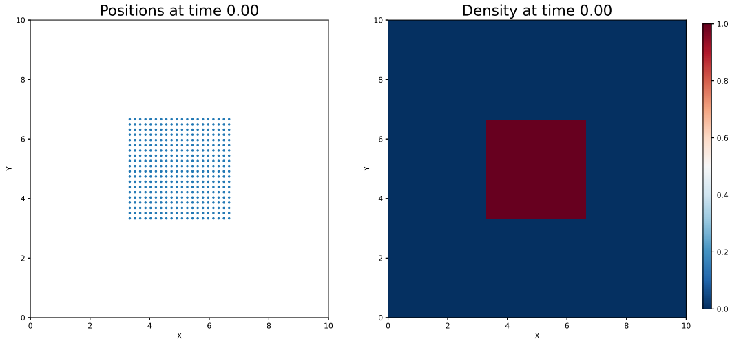
Figure 3.8: Drone swarm particle (left, N = 500 ) and fluid (right) simulations at t = 0s .
