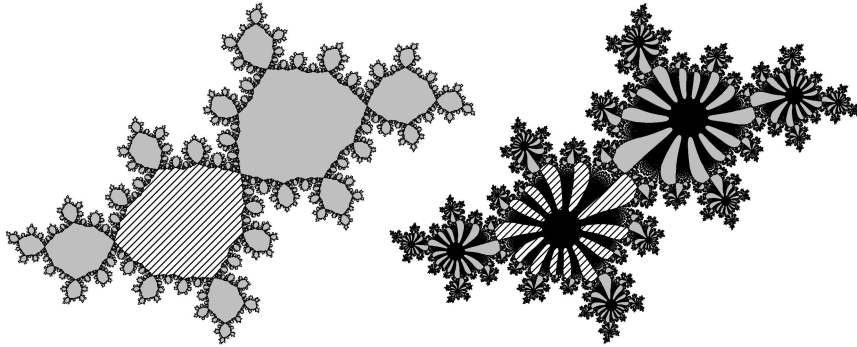
FIGURE 22. Two filled-in Julia sets K_\alpha and K_{\alpha'} , with \alpha' a well-chosen perturbation of \alpha as in Prop. 20. This proposition asserts that if \alpha and \alpha' are chosen carefully enough, P_{\alpha'} has a periodic Siegel disk and the loss of measure from K_\alpha to K_{\alpha'} is small. Left: we hatched the fixed Siegel disk. Right: we hatched the cycle of Siegel disks.
