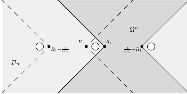
FIGURE 14. The domain \mathcal{D}_n (grey) is the complement of a union of disks and the hourglass \Omega^n (dark grey) is contained in \mathcal{D}_n .
