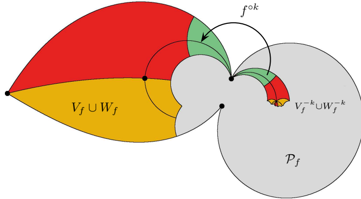
FIGURE 17. If k is large enough, V_f^{-k} \cup W_f^{-k} is contained in the perturbed petal \mathcal{P}_f .
