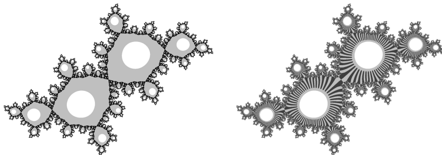
FIGURE 21. Two sets L_\alpha(\rho) and L_{\alpha'}(\rho) , with \alpha' a well-chosen perturbation of \alpha as in Prop. 19. This proposition asserts that if \alpha and \alpha' are chosen carefully enough, the loss of measure from L_\alpha(\rho) to L_{\alpha'}(\rho) is small. We colored white the basin of infinity, the invariant subdisks \Delta_\alpha(\rho) and \Delta_{\alpha'}(\rho) and their preimages; we colored light grey the remaining parts of the Siegel disks and their preimages; we colored dark grey the pixels where the preimages are too small to be drawn.
