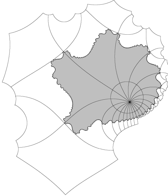
FIGURE 19. If f \in \mathcal{IS}_\alpha with \alpha \in \text{Irrat}_{\geq N} , the set U_1(f) contains the postcritical set \mathcal{PC}(f) . If \alpha is of bounded type, this post-critical set is dense in the boundary of the Siegel disk of f .
