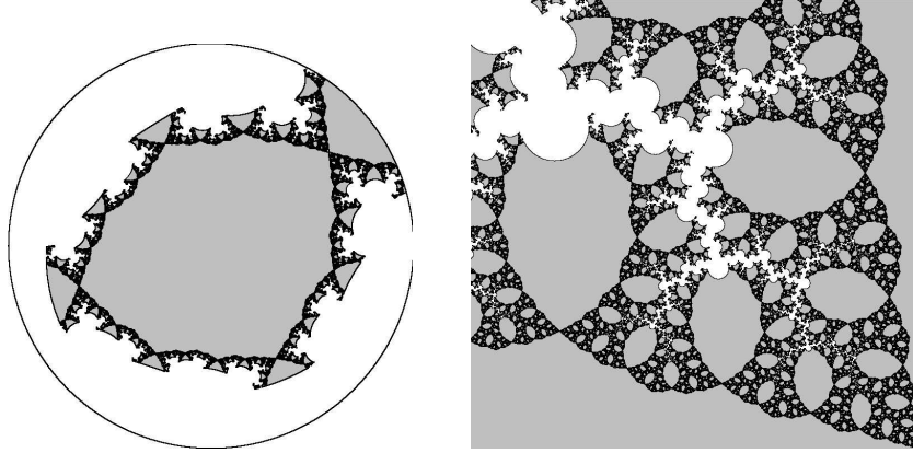
FIGURE 20. If \alpha = (\sqrt{5}-1)/2 , the critical point of P_\alpha is a Lebesgue density point of the set of points whose orbit remain in D(0,1) . Left: the set of points whose orbit remains in D(0,1) . Right: a zoom near the critical point.
