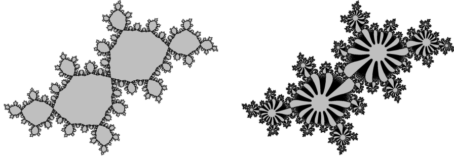
FIGURE 1. Two filled-in Julia sets K_{\alpha} and K_{\alpha'} , with \alpha' a well-chosen perturbation of \alpha as in Prop. 1. This proposition asserts that if \alpha and \alpha' are chosen carefully enough the loss of measure from K_{\alpha} to K_{\alpha'} is small.
