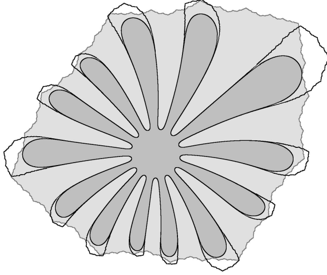
FIGURE 3. Illustration of Prop. 6 for \alpha = \theta = [0, 1, 1, \dots] , n = 7 and A_n = 10^{10} . We see the Siegel disk \Delta of P_\alpha (light grey), the Siegel disk \Delta'_n of the restriction of P_{\alpha_n} to \Delta (dark grey) and the boundary of the Siegel disk of P_{\alpha_n} .
