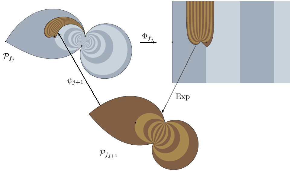
FIGURE 18. The branch \psi_{j+1} maps \mathcal{P}_{f_{j+1}} univalently into \mathcal{P}_{f_j} .
