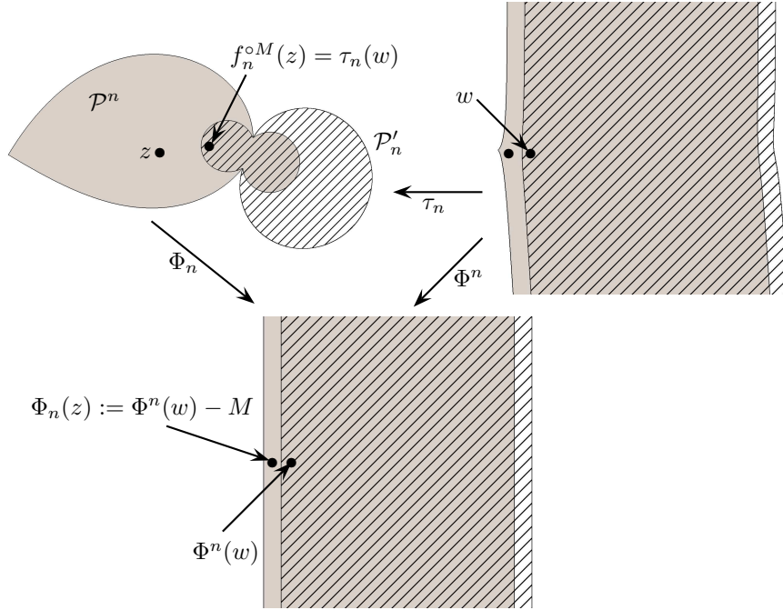
FIGURE 16. Definition of the perturbed Fatou coordinate \Phi_n . The perturbed petal \mathcal{P}_n is grey and the set \mathcal{P}'_n is hatched.
