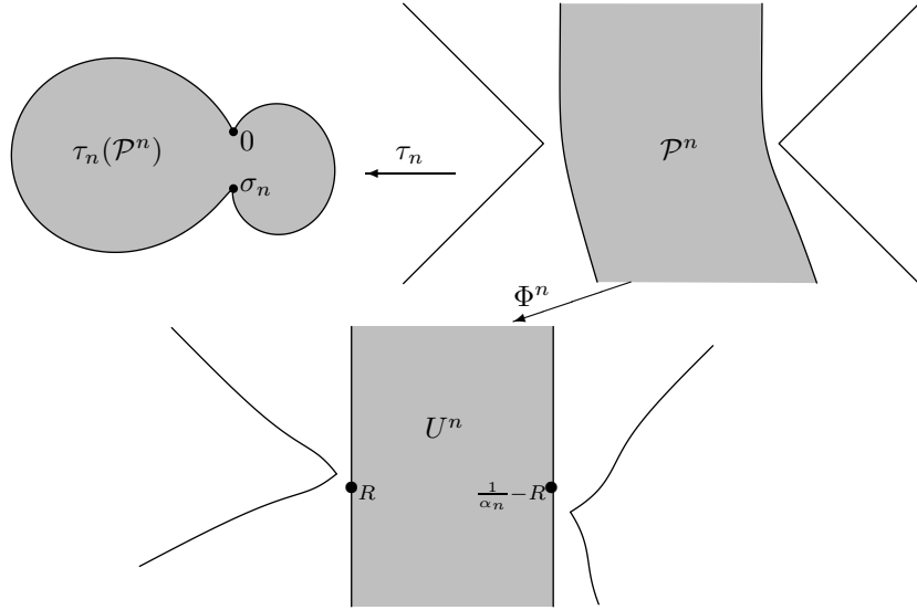
FIGURE 15. The map \tau_n is injective on \mathcal{P}^n := (\Phi^n)^{-1}(U^n) .
