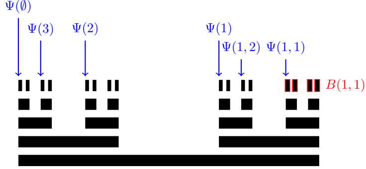
Figure 1: Mapping between \bar{\mathcal{U}} and the Cantor ternary set
