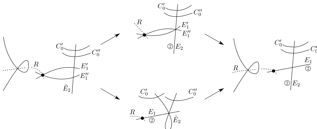
Figure 9: Removing the multiplicities, \bar{\mathcal{C}}_2 \rightarrow \tilde{\mathcal{C}}_2
