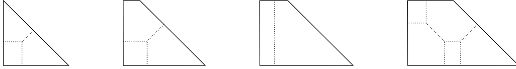
Figure 27: Curves linearly equivalent to H in \mathbf{P}^2 , H in \mathbf{F}_1 , F in \mathbf{F}_1 , and H + F in \mathbf{F}_1 (in the notation introduced in (0.1))
