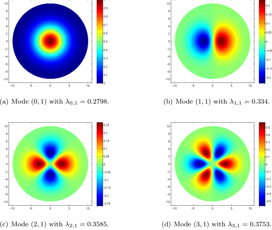
FIGURE 3. Plot of solution of the form \mathcal{P}_{l_{m,n}}^m(\cosh(\tau)) \cos(m\theta) with (\tau, \theta) \in [0, \omega] \times [0, 2\pi] and l_{m,n} = -\frac{1}{2} + i\lambda_{m,n} .
