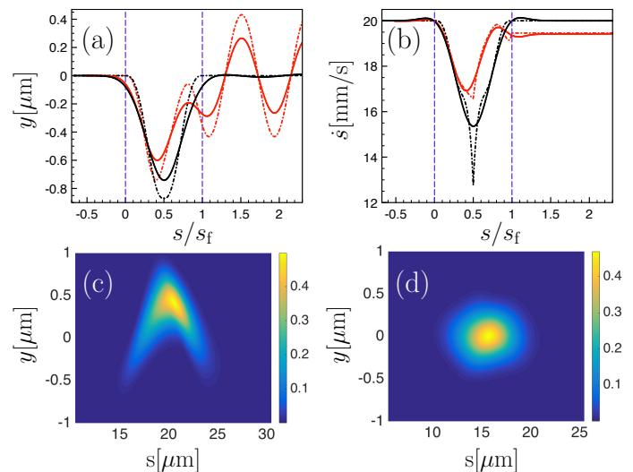
FIGURE 4: (a) and (b) : Transverse position, \langle y(s/s_f) \rangle , and longitudinal velocity, \langle \dot{s} \rangle(s/s_f) , of the wave packet as a function of the normalized longitudinal coordinate, s/s_f . The curves are obtained from 2D classical simulations using either the 1D-adiabatic design (red dot-dashed line) or the 2D-optimized protocol (black dot-dashed line), or from the 2D Schrödinger equation (1) using either the 1D-adiabatic design (red solid line) or the 2D-optimized protocol (black solid line). Color plot of the modulus square of the 2D wavefunction |\phi(s, y)|^2 (in \mu\text{m}^{-2} ) after propagation at the position s = 1.5s_f for the 1D-adiabatic design (c) and 2D-nonadiabatic design (d). Parameters : initial Gaussian wave-function of widths \sigma_y = \sigma_s/10 = (\hbar/m\omega)^{1/2} centered on axis ( y = 0 ) at s = -0.5s_f and with a velocity \dot{s}_0 = 20 \text{ mm/s} .
