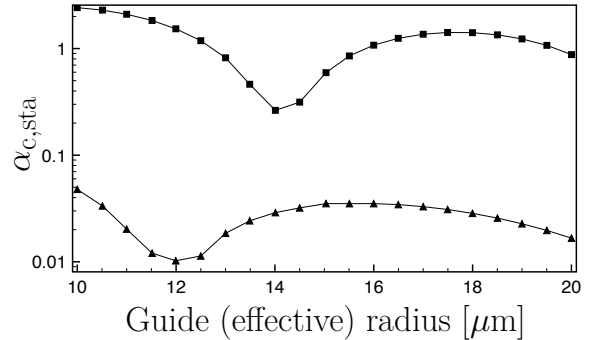
FIGURE 3: Averaged oscillation amplitudes \bar{a}_{\text{sta}} for the engineered guides (triangle) and \bar{a}_c for the circular guides (square) after a right turn as a function of the guide radius. Same initial longitudinal velocity and trapping frequency as for Fig. 2.
