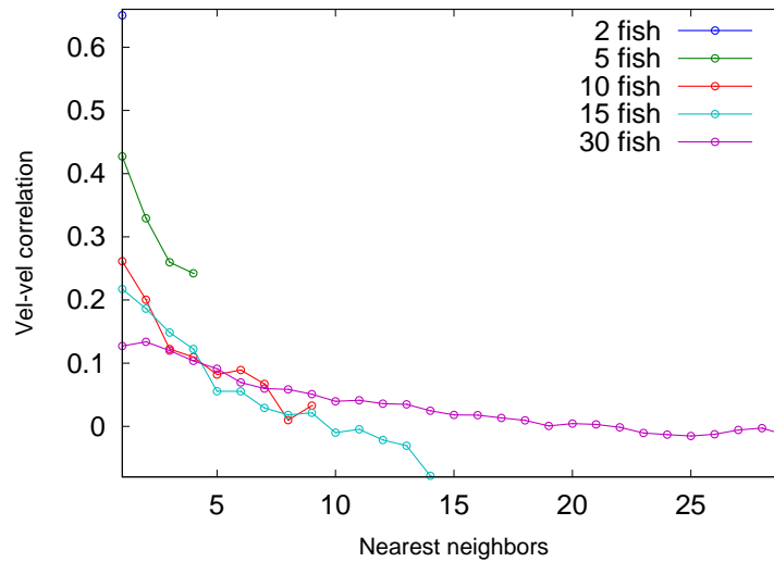
Figure 5.22: The alignment between a fish and its nearest neighbors for different group sizes. We compute the mean of the scalar product between normalized vector speed. The alignment decreases as we take into account farther neighbors.
