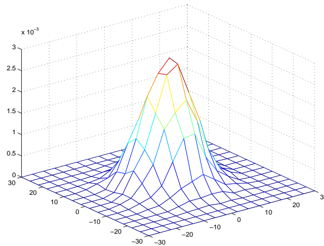
Figure 2.5: The spatial distribution n for \alpha = 2 at time T = 30 time units.
