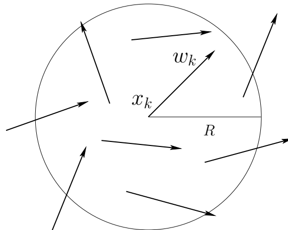
Figure 8: The Vicsek model: each particle updates its velocity with the average velocity of the particles around it. The disc with radius R determines which are the particles taken into account in the estimation of the average velocity.
