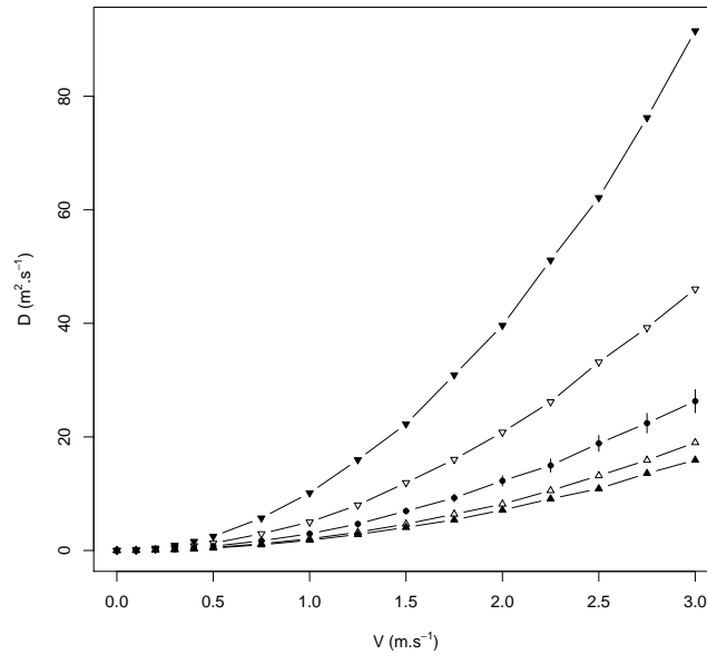
Figure 1.6: Diffusion coefficient D for the PTW model as a function of the swimming speed V , and for different values of the autocorrelation time \tau , but keeping the variance \frac{\tau\sigma^2}{2} of W constant ( \nabla : \tau = \tau^*/4 ; \nabla : \tau = \tau^*/2 ; \bullet : \tau = \tau^* = 0.6 s; \triangle : \tau = 2\tau^* ; \blacktriangle : \tau = 4\tau^* ). Each value was estimated by the Monte-Carlo method, with 10,000 replicates of individual trajectories simulated with \Delta t = 0.01 s over 1200 s and with random initial conditions (heading and turning speed). D was estimated by linear regression from the mean square displacement restricted to the time interval [600..1200] s in order to avoid the ballistic part of the curve. Bars denote the 0.95 confidence interval for the case \bullet : \tau = \tau^* .
