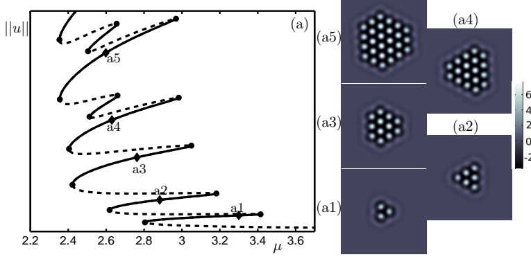
FIG. 4.5. Snaking of patterns with D3 symmetry built around a triangular-organised, three-spot solution. Line style conventions as in Fig. 4.2. Parameters given at the beginning of Sec. 4.2.
