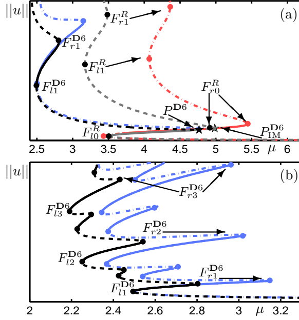
FIG. 4.3. Comparison between the solution branches of PDE4 and IM. Black curves and grey correspond to the PDE approximation and have the line style and labelling conventions as Fig. 4.2. Corresponding radial and D6 solution branches from IM are plotted as dash-dot curves in red and blue, respectively; stability is not indicated and folds not labelled on these branches. (a): Detail close to the spatial-symmetry-breaking bifurcation P^{\mathbf{D6}} ; the corresponding bifurcation for IM is labelled P_{\text{IM}}^{\mathbf{D6}} . (b): Detail of the D6 snaking structure. Parameters given at the beginning of Sec. 4.2.
