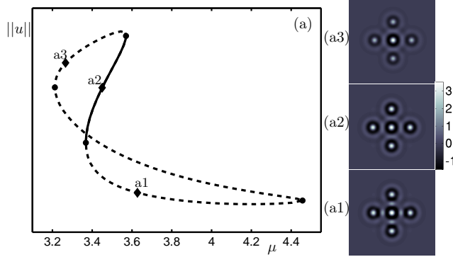
FIG. 4.7. Isola of five-spot solution organised in a quincunx configuration. Line style conventions as in Fig. 4.2. Parameters given at the beginning of Sec. 4.2.
