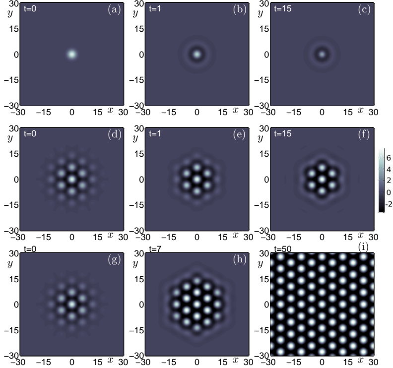
FIG. 1.2. Steady states of the integral model (1.1) posed on the plane, with radially-symmetric connectivity function and sigmoidal firing rate function given by Eq. (1.2); in all simulations \theta = 5.6 , b = 0.4 . (a)–(c): Convergence of a small bump of activity, given by Eq. (A.1), to a spot solution with \mu = 3.4 ; time as indicated in panels. (d)–(f): Convergence of a hexagonal pattern, given by Eq. (A.2), to a stable D6 -symmetric localised state with \mu = 3.2 . (g)–(i) With the same initial condition as (d), divergence away from a localised state to a periodic state with \mu = 3.4 .
