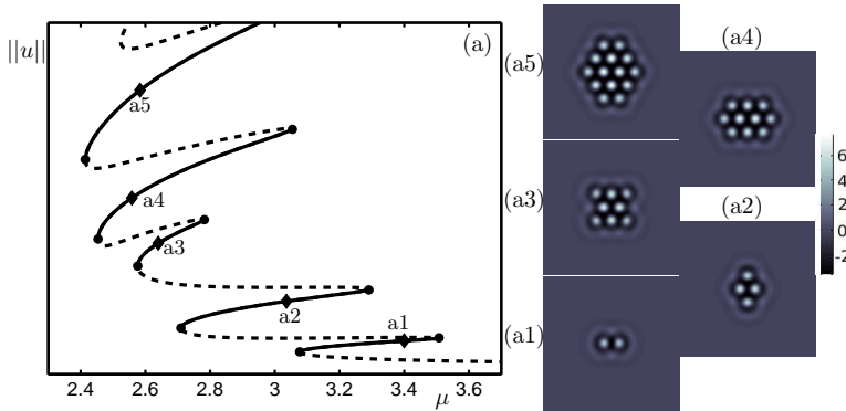
FIG. 4.6. Snaking of patterns with D2 symmetry built around a two-spot solution. Line style conventions as in Fig. 4.2. Parameters given at the beginning of Sec. 4.2.
