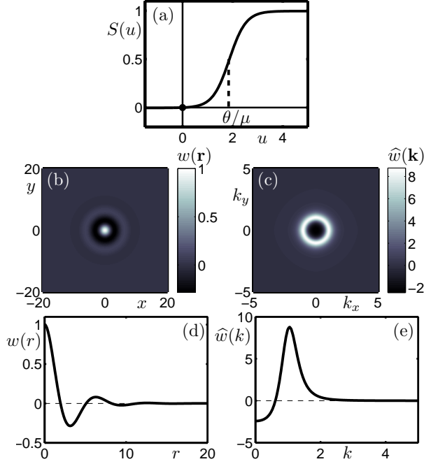
FIG. 2.1. Firing rate function and connectivity function for the integral model. (a): Sigmoidal nonlinearity given by Eq. (2.2) plotted here with \theta = 5.6 and \mu = 3 . (b): Radially-symmetric connectivity kernel given by Eq. (2.3) plotted on the Euclidean plane with b = 0.4 . (c): Its Fourier transform plotted on the (k_x, k_y) -plane. (d): Radial cross section of panel (b). (e): Radial cross section of panel (c).
