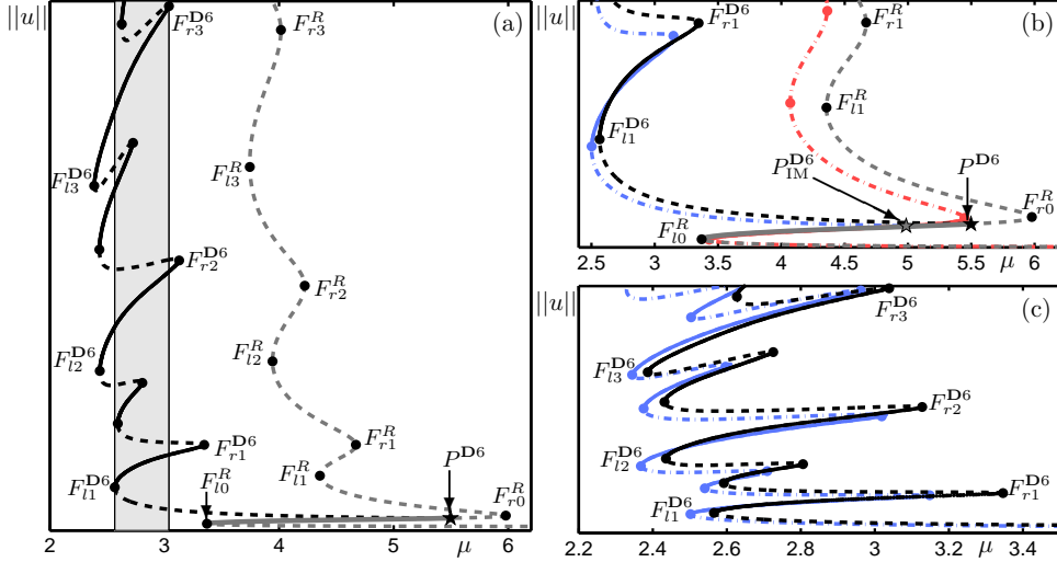
FIG. 4.4. Snaking of radially- and D6 -symmetric localised solutions in terms of \mu for PDE8 and comparison with IM. Black and grey curves correspond to the PDE approximation and have the line style and labelling conventions as Fig. 4.2. Corresponding radial and D6 solution branches from the full model are plotted as dash-dot curves in red and blue, respectively; stability is not indicated and folds not labelled on these branches. (a): Global snaking diagram for PDE8. (b): Detail close to the spatial-symmetry-breaking bifurcation P^{\text{D6}} ; the corresponding bifurcation in the full model is labelled P_{\text{IM}}^{\text{D6}} . (c): Detail of the D6 snaking structure. Parameters given at the beginning of Sec. 4.2.
