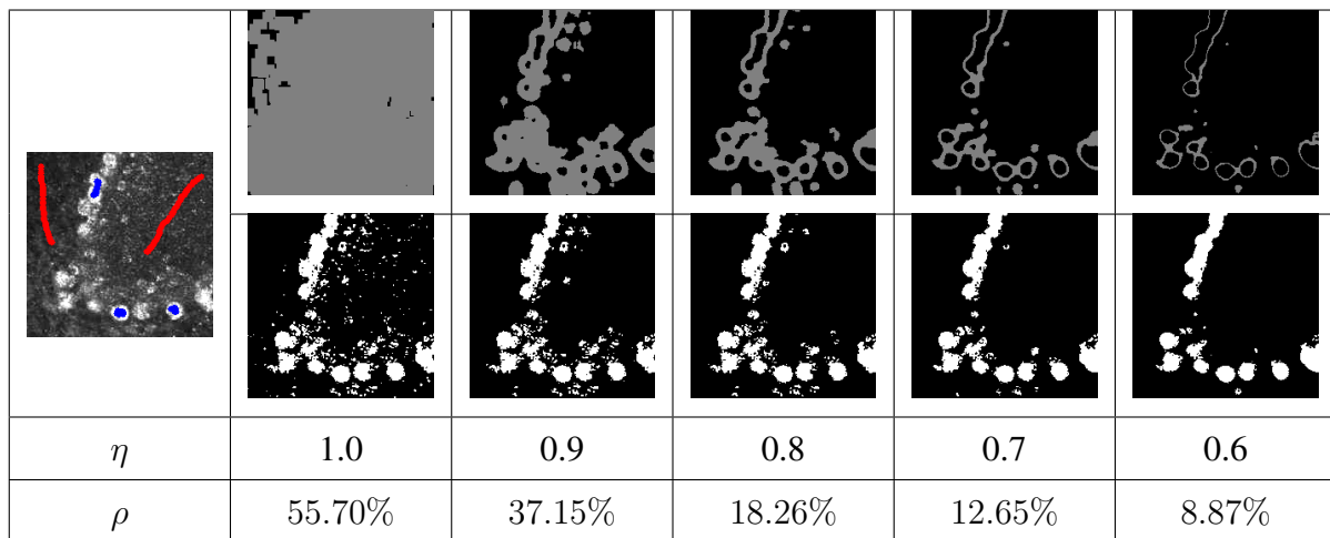
Fig. 12: Simultaneous segmentation and denoising of a 3D image using a Boykov-Jolly model (left) in connectivity 1. In this picture, white spots correspond to cell nuclei in a mouse cerebellum. Top row shows the nodes of the reduced graph in light gray while bottom row shows the corresponding segmentation. In this experiment, we set r = 5 and \gamma = 1 . figure
