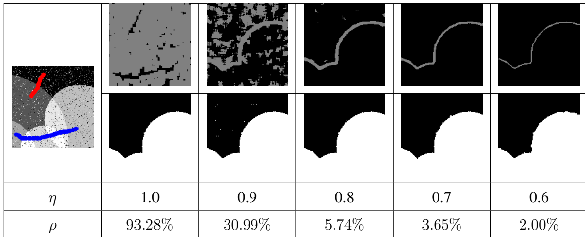
Fig. 11: Memory gain when segmenting a 2D synthetic image corrupted by 10% of impulsive noise, using a Boykov-Jolly model (left). Top row shows the nodes of the reduced graph in light gray while bottom row shows the corresponding segmentation. In this experiment, we set r = 3 , \gamma = 1 and use connectivity 1. In this experiment, \eta_{min} \simeq 0.571 . figure
