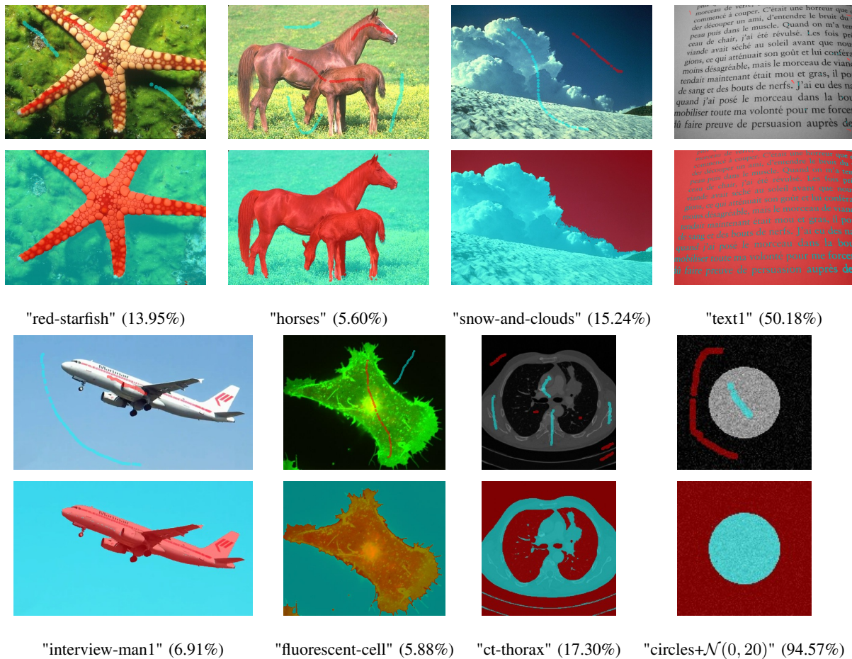
Fig. 8: Segmentation results using a Boykov-Jolly model in connectivity 1. The segmentation (bottom row) as well as seeds (top row) are superimposed on the original image by transparency. The minimal relative size of the reduced graph is indicated in parenthesis below each image figure
