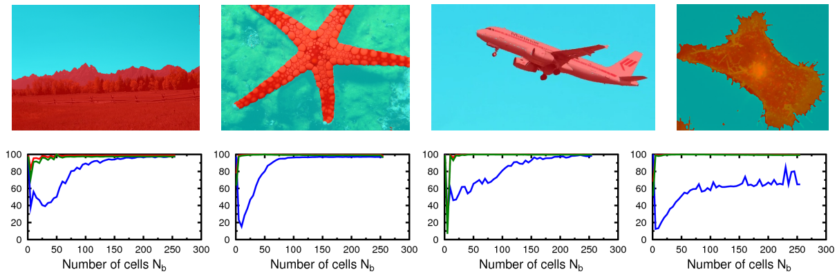
Fig. 6: Evolution of the relative size of the reduced graph (blue curve) and the distance between a ground truth image obtained from Table II with the number of bins N_b . The distance between both segmentations is measured with the DSC (red curve) and the SRMSSD (green curve). Seeds and parameters are the same as those used in Table II.
