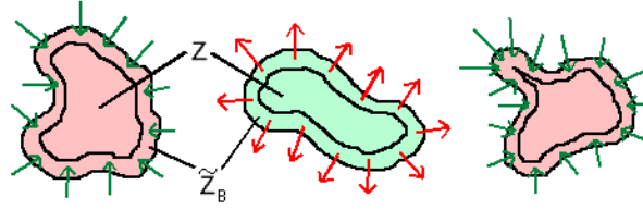
Fig. 2: Principle of the reduction. Red area and arrows (resp. green area arrows) denote the flow which get in (resp. out of) Z_B . The nodes from Z are removed since Z satisfies (10). Remaining nodes are typically located in the narrow band Z_B \setminus Z . figure
