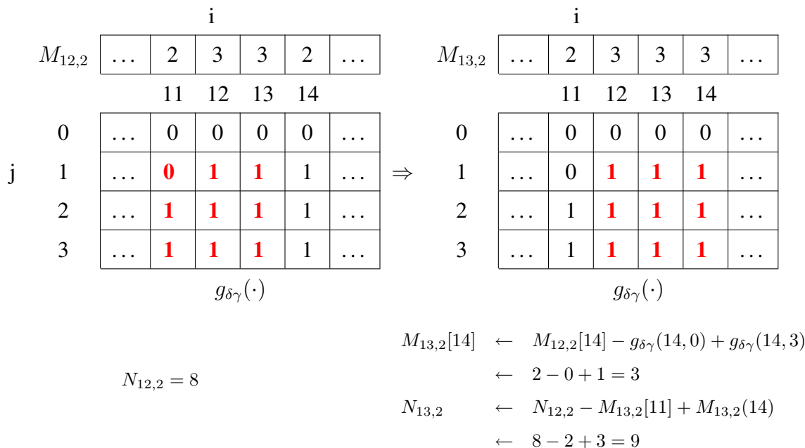
Fig. 4: Illustration of the incremental algorithm for a 2D image with r = 1 , \gamma = 1 and \eta = 1 . In this example, only the node corresponding to the pixel p = (13, 2) is added to \mathcal{G}' since |N_{13,2}| = (2r + 1)^2 = 9 . figure
