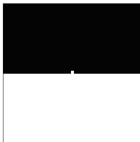
Figure 8: initial condition for the Rayleigh-Taylor instability
