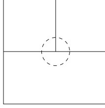
FIGURE 1. Example of a geometrically non-conformal mesh.
