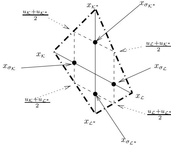
FIG. 4.1. Affine function whose gradient is \nabla_{\mathcal{D}}^{\mathcal{T}} u^{\mathcal{T}}
