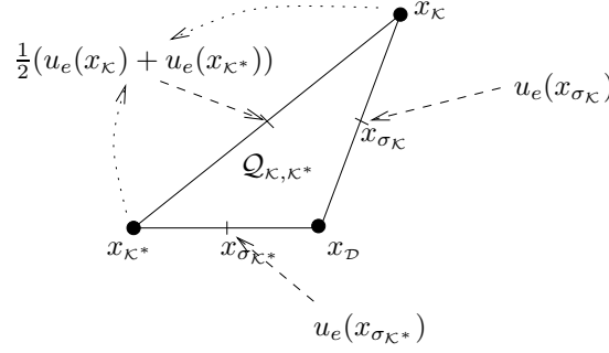
FIG. 5.1. The affine interpolation \mathbb{P}_{\mathcal{Q}_{K,K^*}}^{\Omega} on the quarter diamond \mathcal{Q}_{K,K^*}
