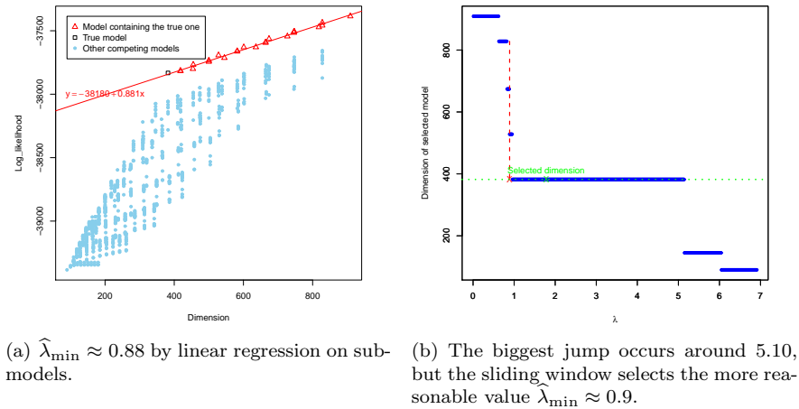
FIG 1. Two ways to compute the slope for a simulated sample of 1000 individuals with 8 clustering loci among 10 and 5 populations. Models are explored via the backward-stepwise method described in Subsection 4.2; the number of clusters K ranges from 1 to 10. The size of the sliding window is 0.10.
