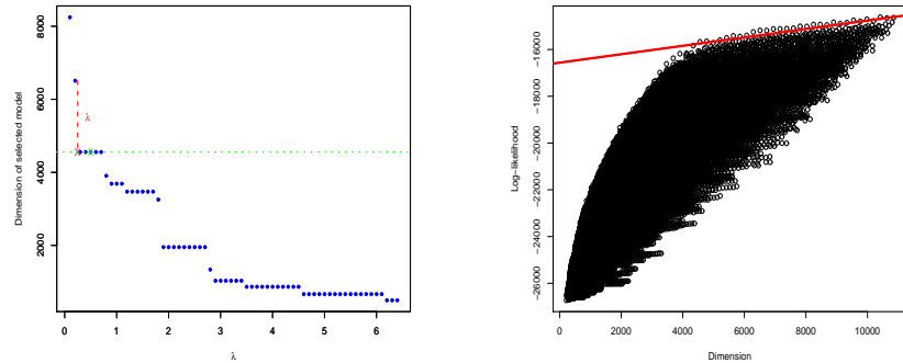
(a) Selected dimension versus candidate constants: the selected constant is \hat{\lambda} = 0.25 , leading to an optimal penalty pen_{opt} = 0.50 * Dimension .
