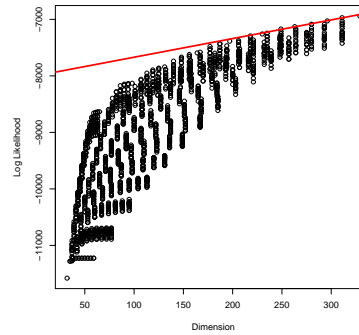
(b) Log-likelihood versus Dimension of the most competitive models from the voting data: the red line corresponds to the equation y = \hat{\lambda}x + \beta .
