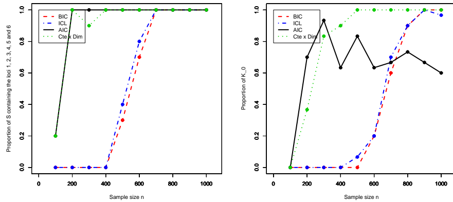
FIG 2. Left: Graph showing the proportion of selected models with \widehat{S}_n containing 1, \dots, 6 with respect to sample size n . Right: Graph showing the proportion of selected models with \widehat{K}_n = K_0 with respect to sample size n .
