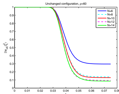
FIGURE 5. Plot of the UC probability as a function of t , for \rho = 60 and several spin-detectors N .
