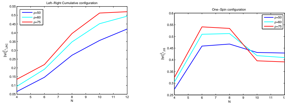
FIGURE 2. Plot of the 2 * LRC and OS probabilities at final time t_* , as a function of N and for \rho = 50, 60, 75 .
