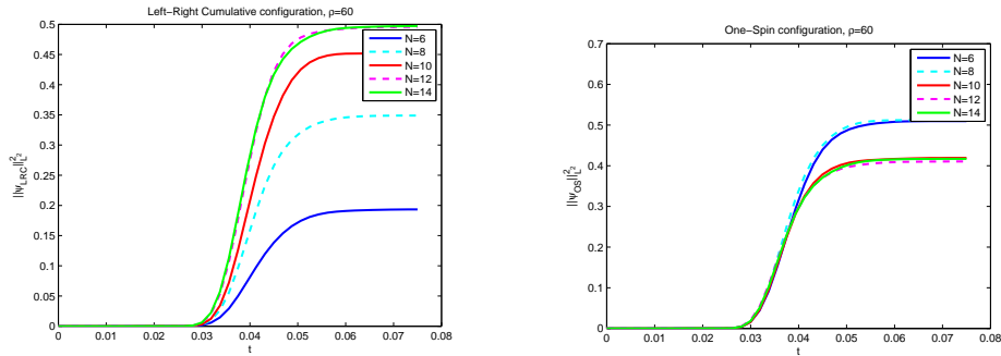
FIGURE 4. Plot of the 2 * LRC and OS probabilities as a function of t , for \rho = 60 and several spin-detectors N .
