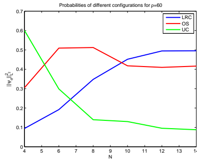
FIGURE 1. Plot of the 2 * LRC , OS and UC probabilities at final time t_* , as a function of N and for \rho = 60 .
