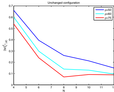
FIGURE 3. Plot of the UC probability at final time t_* , as a function of N and for \rho = 50, 60, 75 .
