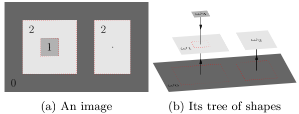
Figure 1: An example of tree of shapes
