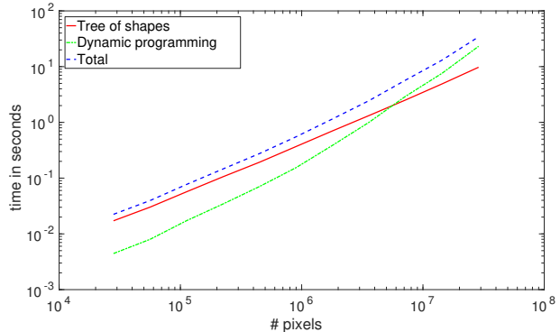
Figure 2: Log-log plot of the computing times in seconds w.r.t. the number of pixels of the image. Red: time to construct the tree of shapes. Green: time to solve the isotonic regression via dynamic programming. Blue: total time for the algorithm (including copies of trees, arrays, etc...).
