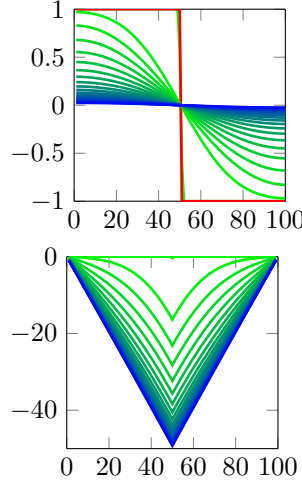
Figure 9: First 20000 iterations of the primal-dual pair (\alpha^{(k)}, \lambda^{(k)}) . Top: \beta is displayed in red while \alpha^{(k)} varies from green to blue with iterations. Bottom: \lambda^{(k)} varies from green to blue with iterations. A new curve is displayed every 1000 iterations. As can be seen, the convergence is very slow.
