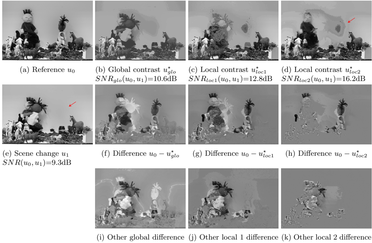
Figure 6: Comparing the different algorithms for different scenes under a similar illumination.
