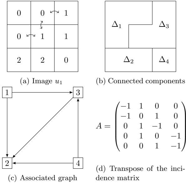
Figure 4: Illustration of the graph construction
