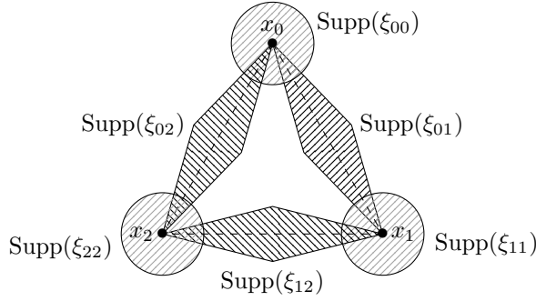
Figure 5: The supports of the \xi_{ij} when d = 2
