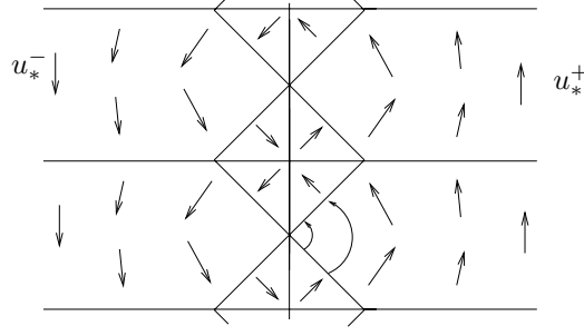
Figure 6: Limit cross-tie wall u_\eta(\alpha) connecting the states u_*^\pm = (0, \pm 1) in a strip of thickness \eta . Here, \alpha \in (0, \frac{\pi}{4}] is the angle of the isosceles triangle, that is equal with half the angle represented by the two circle arrows.
