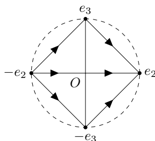
Figure 4: Geodesics in the plane \{z_1 = 0\}
