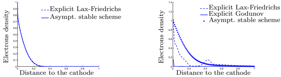
Figure 2. Plasma expansion: electron density, at time t = 5.10^{-1} . Left figure: explicit Lax-Friedrichs scheme and asymptotically stable scheme with \Delta x = 10^{-4} and w_p \Delta t \leq 1 (Debye length and plasma frequency are fully resolved ). Right figure: explicit Lax-Friedrichs and Godunov schemes and asymptotically stable scheme with \Delta x = 10^{-2} and w_p \Delta t > 1 (Debye length and plasma frequency are not resolved ).
