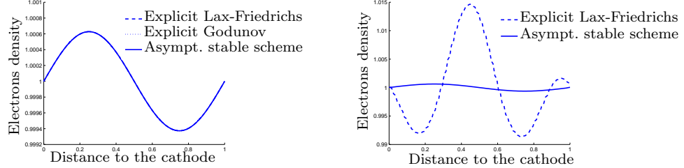
Figure 1. Perturbation of a uniform plasma: electron density, at time t = 10^{-2} . Left figure: explicit Lax-Friedrichs and Godunov schemes and asymptotically stable scheme with \Delta x = 10^{-4} and w_p \Delta t \leq 1 (Debye length and plasma frequency are fully resolved ). Right figure: explicit Lax-Friedrichs scheme (explicit Godunov scheme fails) and asymptotically stable scheme with \Delta x = 10^{-2} and w_p \Delta t > 1 (Debye length and plasma frequency are not resolved ).
