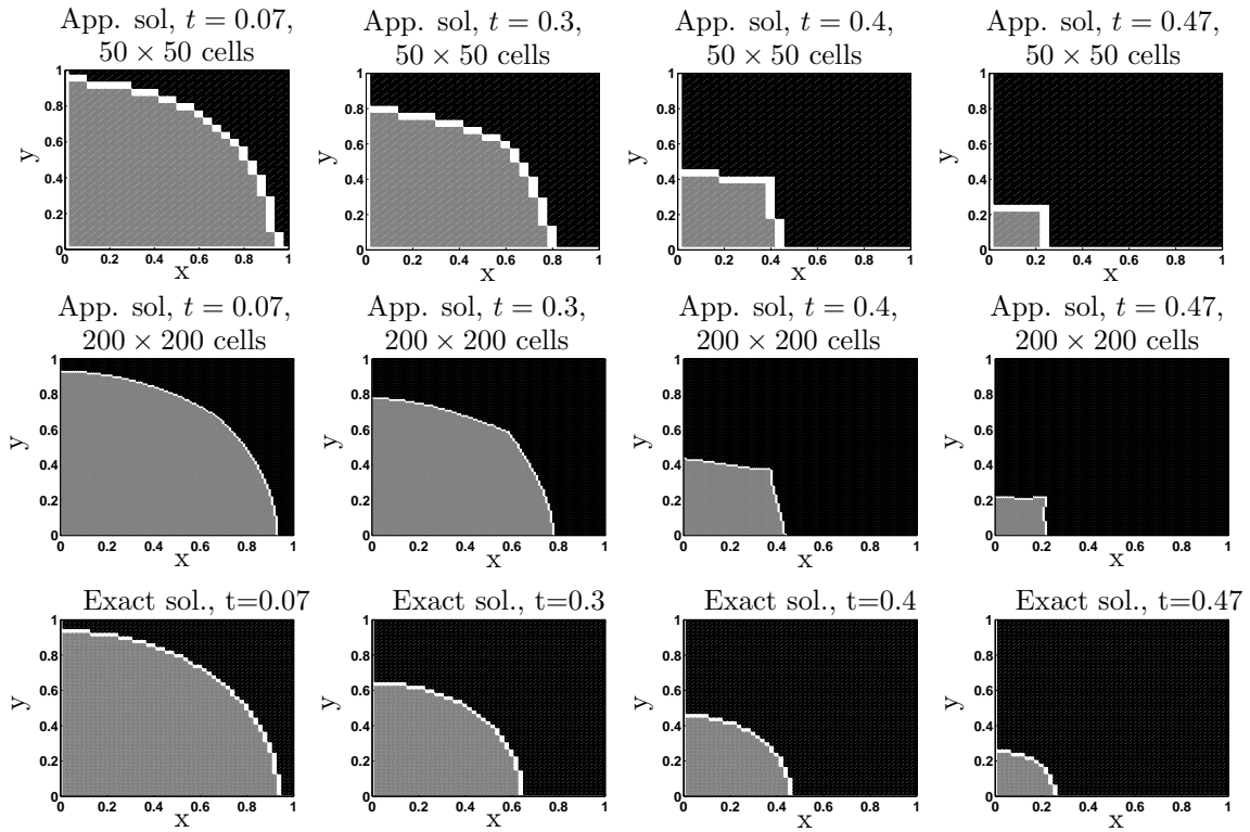
Figure 14: Fluid bubble for different times t = 0.07 , t = 0.3 , t = 0.4 and t = 0.47 . We can see the different type of the cells: in gray, the full cells, in white, the mixed cells and in black, the empty cells. Top and middle, the results are computed with the V.O.F. scheme presented in Section 3 with \Delta x = \Delta y = 2/50 (top) and \Delta x = \Delta y = 2/200 (middle). Bottom: the results are computed with the exact solution given by (23) and projected on the mesh.
