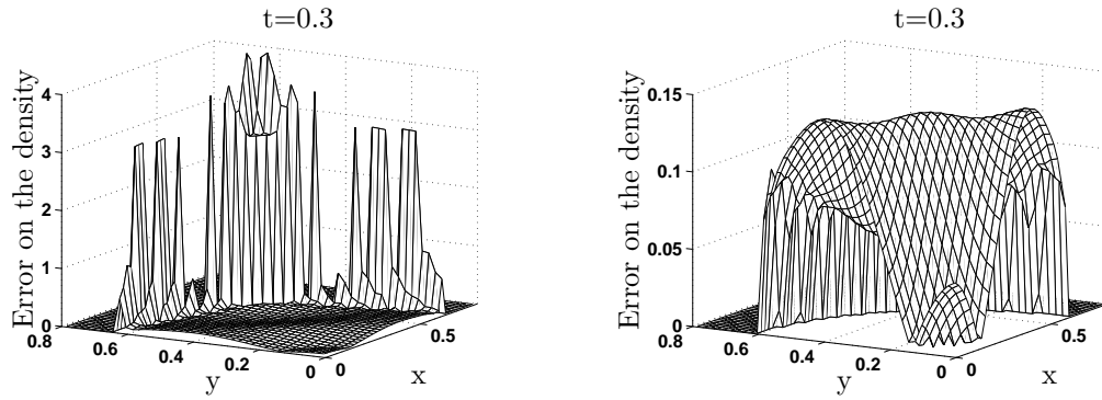
Figure 12: Difference between the exact and the approximate densities at time t = 0.3 , on the left for all the fluid bubble and on the right only for interior cells. The approximate density is given by the V.O.F. scheme presented in Section 3 for \Delta x = \Delta y = 2/100 . The exact density is given by (23) and is projected on the mesh.
