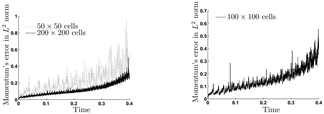
Figure 8: L^2 relative error on the fluid momentum as a function of time for different meshes: \Delta x = \Delta y = 2/50 and \Delta x = \Delta y = 2/200 (left) and \Delta x = \Delta y = 2/100 (right). The “100 × 100 cells” curve is between the “200 × 200 cells” and “50 × 50 cells” curves.
