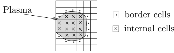
Figure 3: Location of border cells for which we have to take into account of the pressure reaction force in the discretization.
