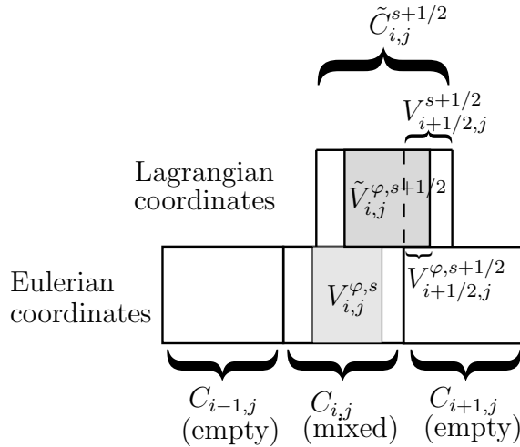
Figure 4: Determination of the plasma volume flowed through \sigma_{i+1/2,j} = \partial C_{i,j} \cap \partial C_{i+1,j} during a time step when C_{i,j} is a mixed cell and C_{i-1,j} and C_{i+1,j} are empty cells.
