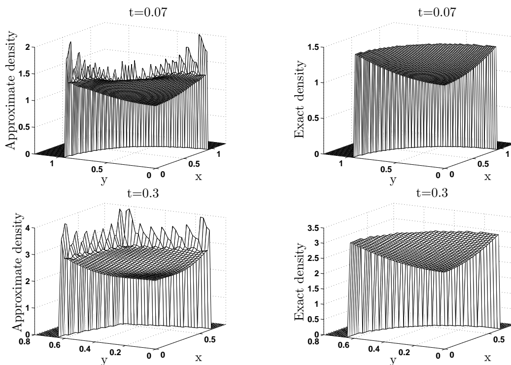
Figure 10: On the left: approximate density given by the V.O.F. scheme presented in Section 3 at times t = 0.07 and t = 0.3 for \Delta x = \Delta y = 2/100 . On the right: exact density given by (23) at times t = 0.07 and t = 0.3 . It is projected on the mesh.
