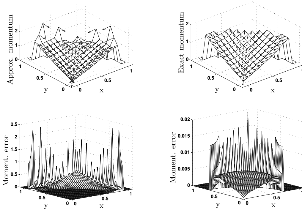
Figure 13: Top: Euclidean norms of the approximate momentum (left) and of the exact momentum (right) at time t = 0.07 . Bottom: Difference between the Euclidean norms of the exact and approximate momentums at time t = 0.07 , on the left for all the fluid bubble, on the right only for interior cells. The approximate momentum is given by the V.O.F. scheme presented in Section 3 for \Delta x = \Delta y = 2/100 . The exact momentum is given by (23) and is projected on the mesh.
