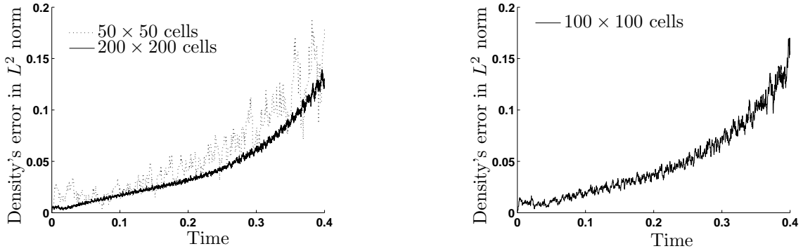
Figure 7: L^2 relative error on the fluid density as a function of time for different meshes: \Delta x = \Delta y = 2/50 and \Delta x = \Delta y = 2/200 (left), \Delta x = \Delta y = 2/100 (right). The “100 × 100 cells” curve is between the “200 × 200 cells” and “50 × 50 cells” curves.
