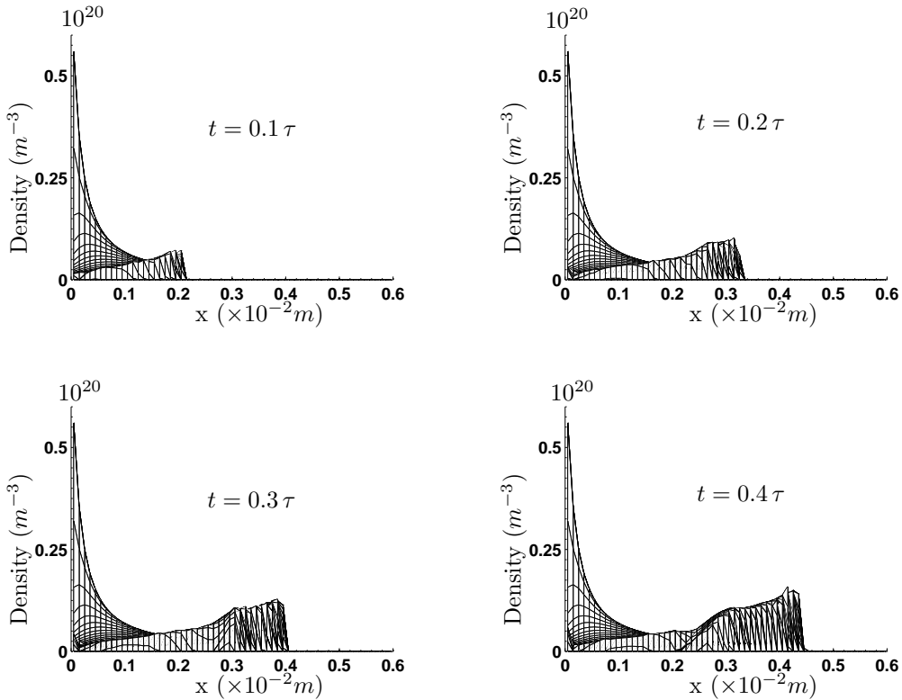
Figure 16: Orthogonal projection on [0, x) of the plasma density at the time t = 0.1\tau , t = 0.2\tau , t = 0.3\tau , t = 0.4\tau with \tau = u_0/L = 6.67 \times 10^{-7} second. The solution is computed with the discretized asymptotic model using the V.OF. scheme presented in Section 3. We use a uniform Cartesian mesh with 100 \times 100 cells.
