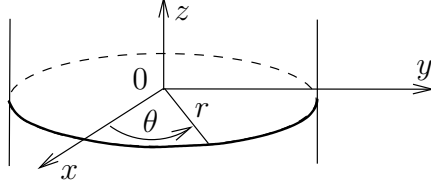
Figure 6: Fluid subject to an external homogeneous space pressure.
