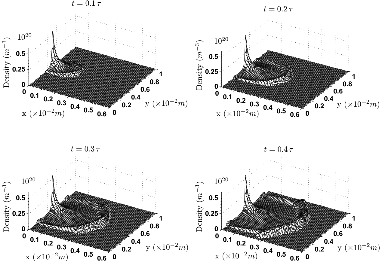
Figure 15: Plasma density at the time t = 0.1\tau , t = 0.2\tau , t = 0.3\tau , t = 0.4\tau with \tau = u_0/L = 6.67 \times 10^{-7} second. The solution is computed with the discretized asymptotic model using the V.OF. scheme presented in Section 3. We use a uniform Cartesian mesh with 100 \times 100 cells.
