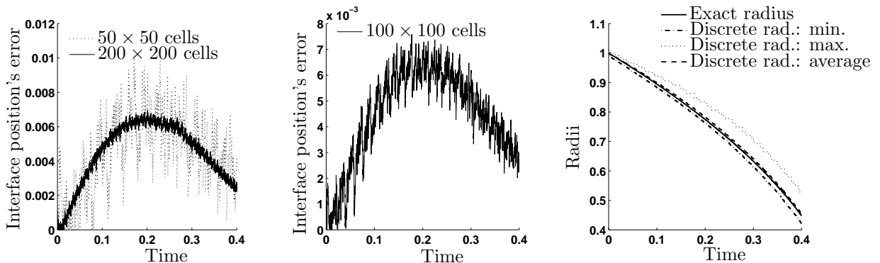
Figure 9: Left and middle: Relative error on the fluid-vacuum interface position, for \Delta x = \Delta y = 2/50 and \Delta x = \Delta y = 2/200 (left) and \Delta x = \Delta y = 2/100 (middle). The approximate values of the fluid-vacuum interface positions are given by the averaged value of the distance between the origin and the center of all border cells (see Fig. 3 for the definition of border cells). The “ 100 \times 100 cells” curve is between the “ 200 \times 200 cells” and “ 50 \times 50 cells” curves. Right: exact and approximate values of the plasma-vacuum interface position as functions of time for \Delta x = \Delta y = 2/100 . The approximate values are the minimum, the maximum and the averaged value of the distance between the origin and the center of all border cells.
