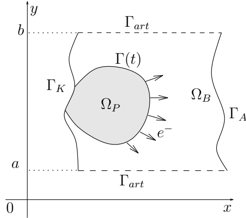
Figure 1: The two-dimensional device: the plasma bubble, \Omega_P , expands between the cathode \Gamma_K and the anode \Gamma_A , during its expansion some electrons are emitted in the vacuum forming a beam in \Omega_B .
