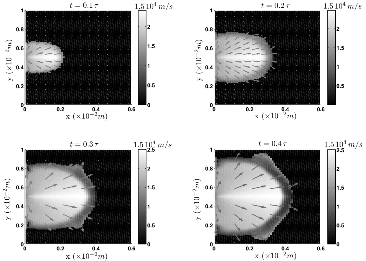
Figure 17: Plasma velocity at the time t = 0.1\tau , t = 0.2\tau , t = 0.3\tau , t = 0.4\tau with \tau = u_0/L = 6.67 \times 10^{-7} second. The solution is computed with the discretized asymptotic model using the V.OF. scheme presented in Section 3. We use a uniform Cartesian mesh with 100 \times 100 cells. The vectors indicate the direction of the velocity vector and the color gives the L^2 norm of the velocity vector.
