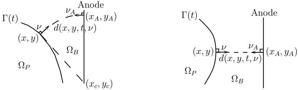
Figure 2: Approximation of the electron trajectory in the simplified Child Langmuir model for the beam region.
