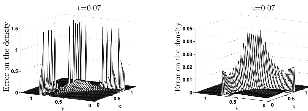
Figure 11: Difference between the exact and the approximate densities at time t = 0.07 , on the left for all the fluid bubble and on the right only for interior cells. The approximate density is given by the V.O.F. scheme presented in Section 3 for \Delta x = \Delta y = 2/100 . The exact density is given by (23) and is projected on the mesh.
