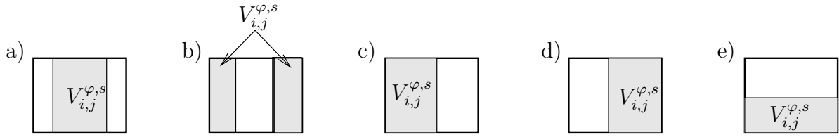
Figure 5: Location of the plasma volume in the cell C_{i,j} in the case a) C_{i-1,j} and C_{i+1,j} are both empty b) C_{i-1,j} and C_{i+1,j} are both full, c) C_{i-1,j} is full and C_{i+1,j} is empty or C_{i-1,j} is full and C_{i+1,j} is mixed or C_{i-1,j} is mixed and C_{i+1,j} is empty, d) C_{i-1,j} is empty and C_{i+1,j} is full or C_{i-1,j} is mixed and C_{i+1,j} is full or C_{i-1,j} is empty and C_{i+1,j} is mixed, e) C_{i-1,j} and C_{i+1,j} are both mixed.
