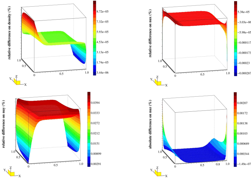
Figure 4: Relative difference between the computed solution and the exact drift-fluid limit of the resolved AP scheme at time t = 0.1 for \varepsilon = 10^{-6} ; density n (top left), x -component of the momentum nu_x (top right), y -component of the momentum nu_y (bottom left). Absolute difference between the computed solution and the exact drift-fluid limit on the z -component of the momentum nu_z (bottom right).
