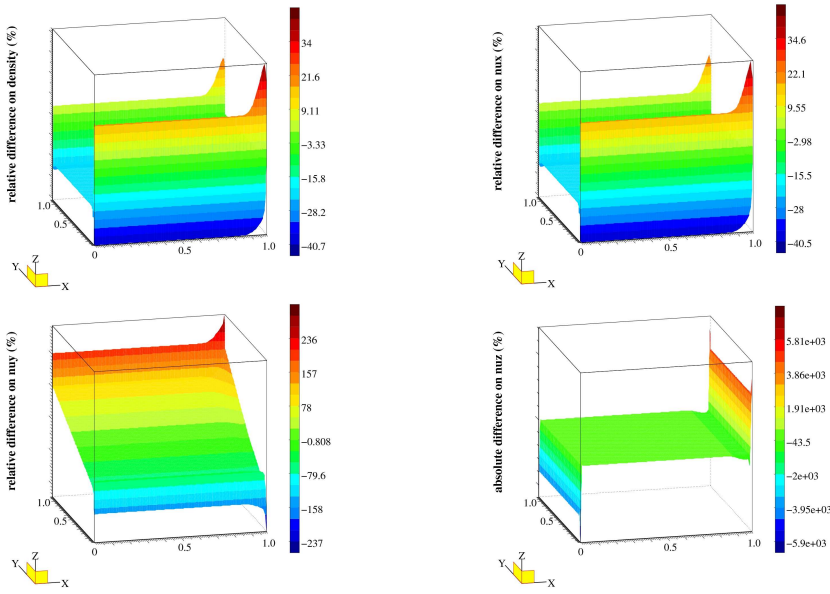
Figure 13: Relative difference between the computed solution and the exact drift-fluid limit of the non-resolved AP scheme at time t = 0.1 for unprepared initial and boundary conditions \varepsilon = 10^{-6} and \varepsilon' = 10^{-2} ; density n (top left), x -component of the momentum nu_x (top right), y -component of the momentum nu_y (bottom left). Absolute difference between the computed solution and the exact drift-fluid limit on the z -component of the momentum nu_z (bottom right).
