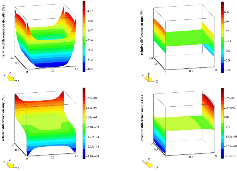
Figure 12: Relative difference between the computed solution and the exact drift-fluid limit of the resolved AP scheme at time t = 0.1 for unprepared initial and boundary conditions \varepsilon = 10^{-6} and \varepsilon' = 10^{-2} ; density n (top left), x -component of the momentum nu_x (top right), y -component of the momentum nu_y (bottom left). Absolute difference between the computed solution and the exact drift-fluid limit on the z -component of the momentum nu_z (bottom right).
