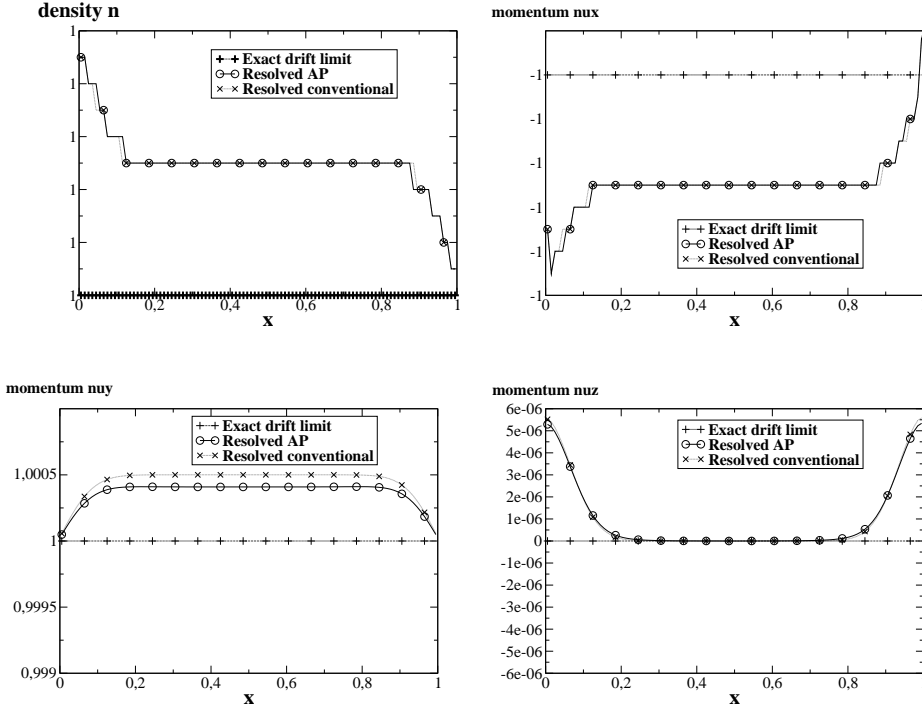
Figure 3: Comparison of the resolved conventional scheme (crosses), the resolved AP scheme (circles) and the exact drift-fluid limit (vertical bars) at t = 0.1 for \varepsilon = 10^{-6} ; density n (top left), x -component of the momentum nu_x (top right), y -component of the momentum nu_y (bottom left), z -component of the momentum nu_z (bottom right).
