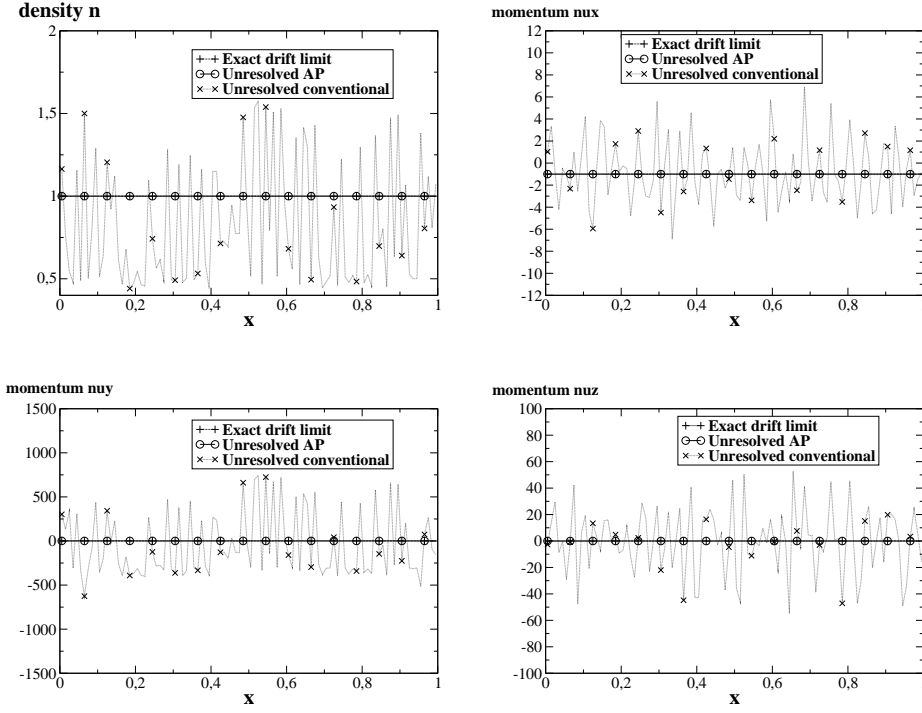
Figure 5: Comparison of the non-resolved conventional scheme (crosses), the non-resolved AP scheme (circles) and the exact drift-fluid limit (vertical bars) at t = 0.1 for \varepsilon = 10^{-6} ; density n (top left), x -component of the momentum nu_x (top right), y -component of the momentum nu_y (bottom left), z -component of the momentum nu_z (bottom right).
