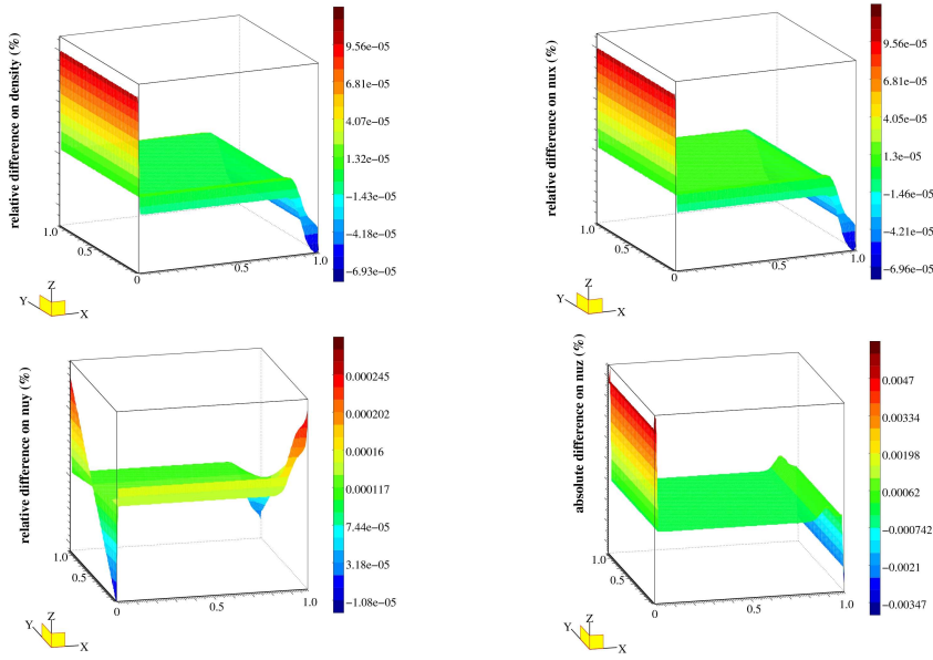
Figure 7: Relative difference between the computed solution and the exact drift-fluid limit of the non-resolved AP scheme at time t = 0.1 for \varepsilon = 10^{-6} ; density n (top left), x -component of the momentum nu_x (top right), y -component of the momentum nu_y (bottom left). Absolute difference between the computed solution and the exact drift-fluid limit on the z -component of the momentum nu_z (bottom right).
