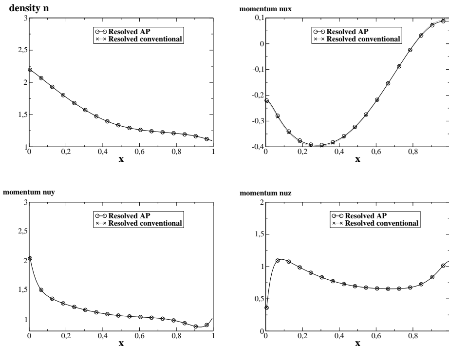
Figure 9: Comparison of the conventional scheme (crosses), and resolved AP scheme (circles) at t = 1 for \varepsilon = 1 ; density n (top left), x -component of the momentum nu_x (top right), y -component of the momentum nu_y (bottom left), z -component of the momentum nu_z (bottom right).
