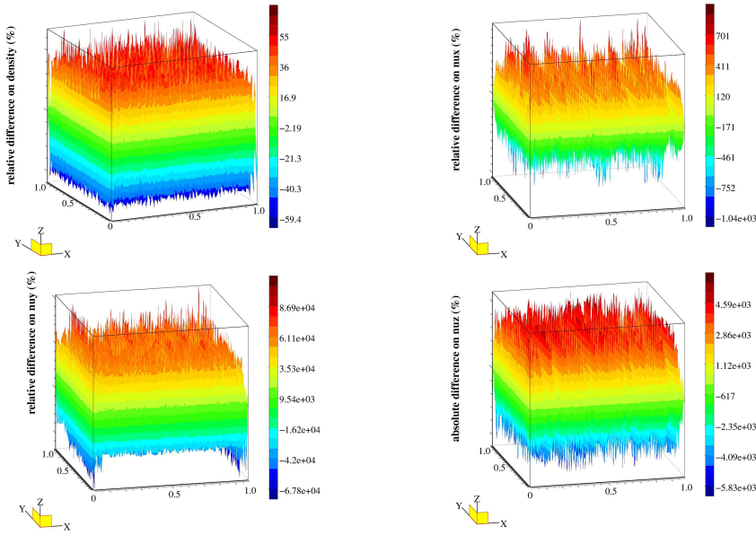
Figure 6: Relative difference between the computed solution and the exact drift-fluid limit of the non-resolved conventional scheme at time t = 0.1 for \varepsilon = 10^{-6} ; density n (top left), x -component of the momentum nu_x (top right), y -component of the momentum nu_y (bottom left). Absolute difference between the computed solution and the exact drift-fluid limit on the z -component of the momentum nu_z (bottom right).
