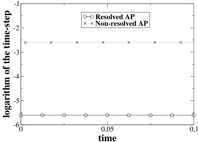
Figure 8: Time-step (log scale) as a function of time for the resolved and non-resolved AP schemes when \varepsilon = 10^{-6} .
