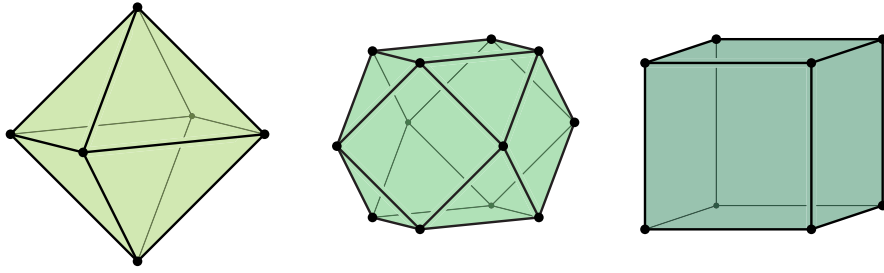
Figure 3. The unit ball B_{(2)}^* between the cross-polytope and the hypercube.
