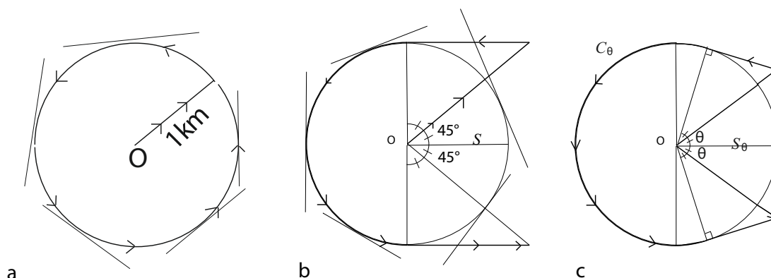
FIGURE 1. Searching for a curve of minimal length.
