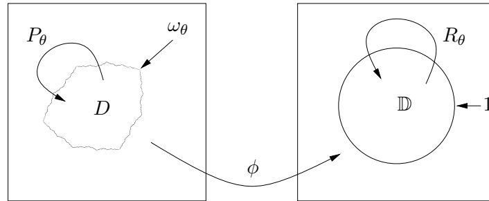
Figure 2: The linearizing map \phi : \bar{D} \rightarrow \bar{\mathbb{D}} sending \omega_\theta to 1.
