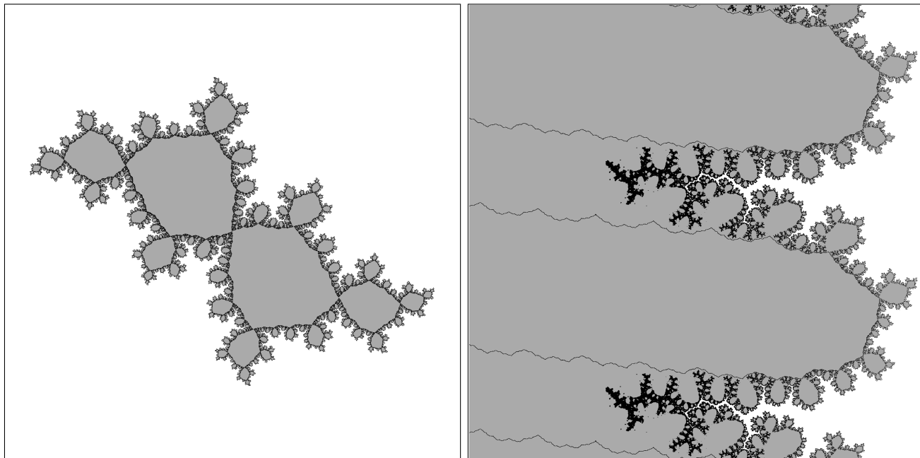
Figure 6: The filled-in Julia set of the polynomial P_\theta , \theta = [2, 1, 2, 1, 2, 1 \dots] and its image under the map \chi_\theta(z) = \log(z - \omega_\theta) .
