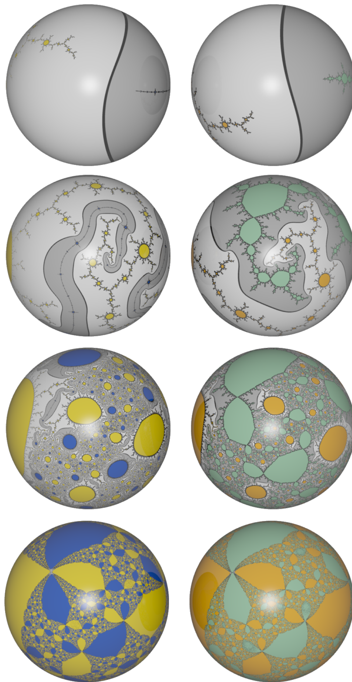
FIGURE 1. A shared mating of two quadratic polynomials having critical points of period 4 (pictures by I. Zidane). The rational map has a period 2 cluster. It can be seen as a geometric mating in 4 distinct ways. Here, we see two of them. Left: mating the left-most real quadratic polynomial of period 4 with the co-kokopelli. Right: mating the bi-basilica with the kokopelli.
