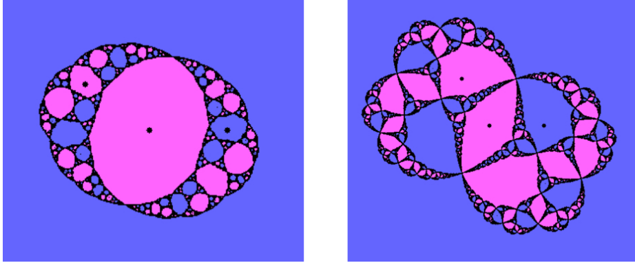
FIGURE 4. Twisted matings of the basilica, P = Q : z \mapsto z^2 - 1 . Left: a geometric mating of P_1^2 and Q_\alpha^2 with \alpha = \exp(-2\pi i/3) . Right: a geometric mating of P_1^4 and Q_\beta^4 with \beta = \exp(-2\pi i/5) .
